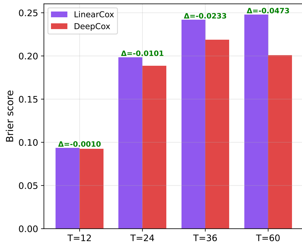
Brier score: lower is better
