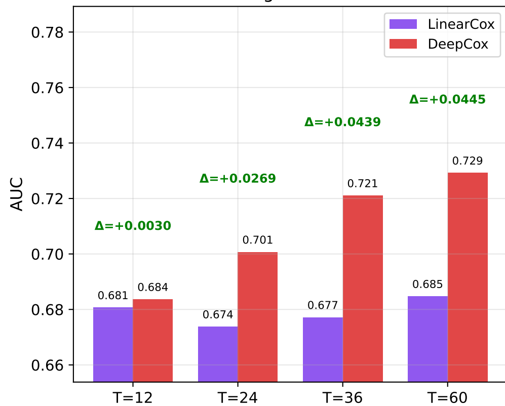
AUC: higher is better
