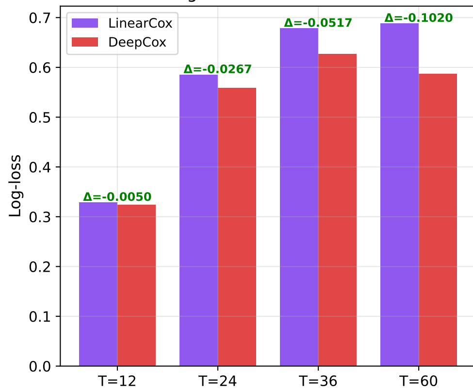
Log-loss: lower is better
